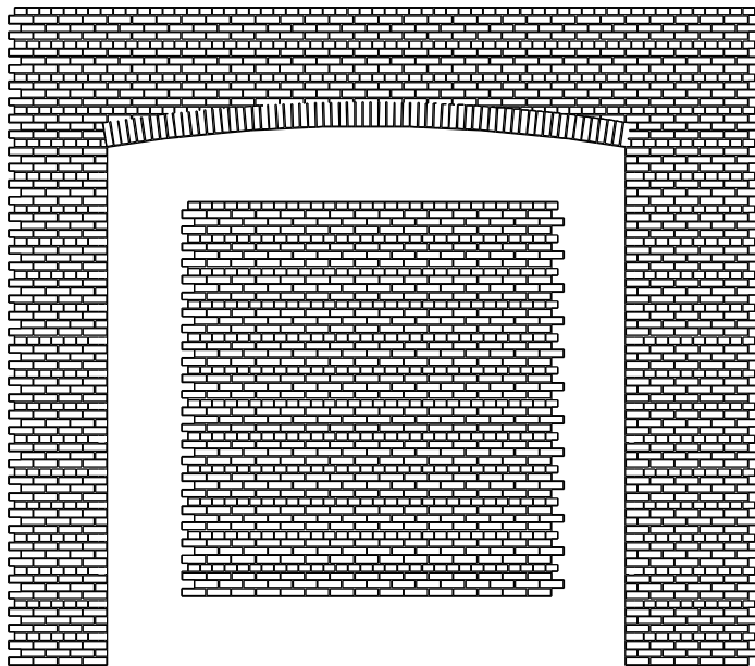
various 48 and 80 brick tall garden wall bond brick sections, fit LCUT windows
